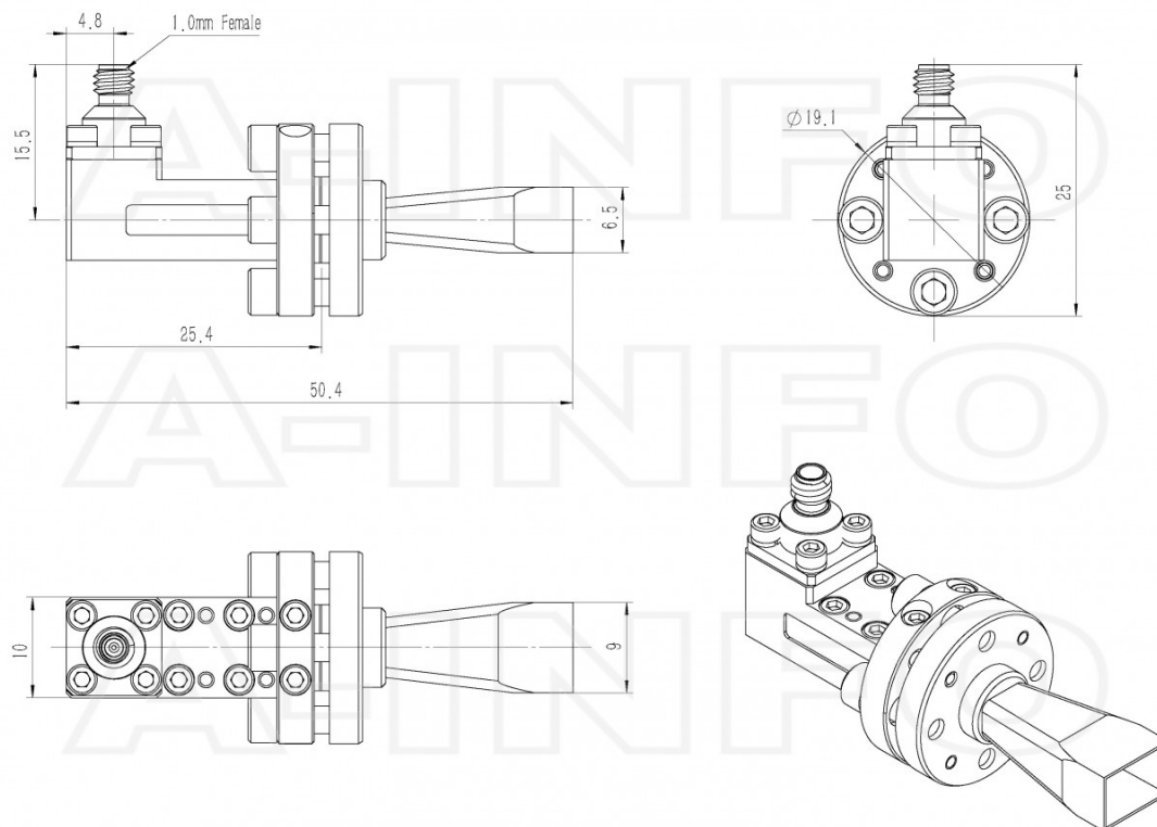
1.0mm-Female Output (P/N: LB-10-15-C-1.0F)
